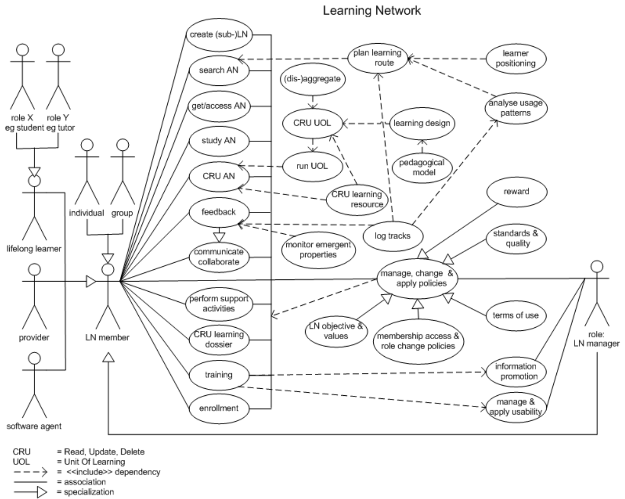
Figure 3: Use case model for Learning Networks
